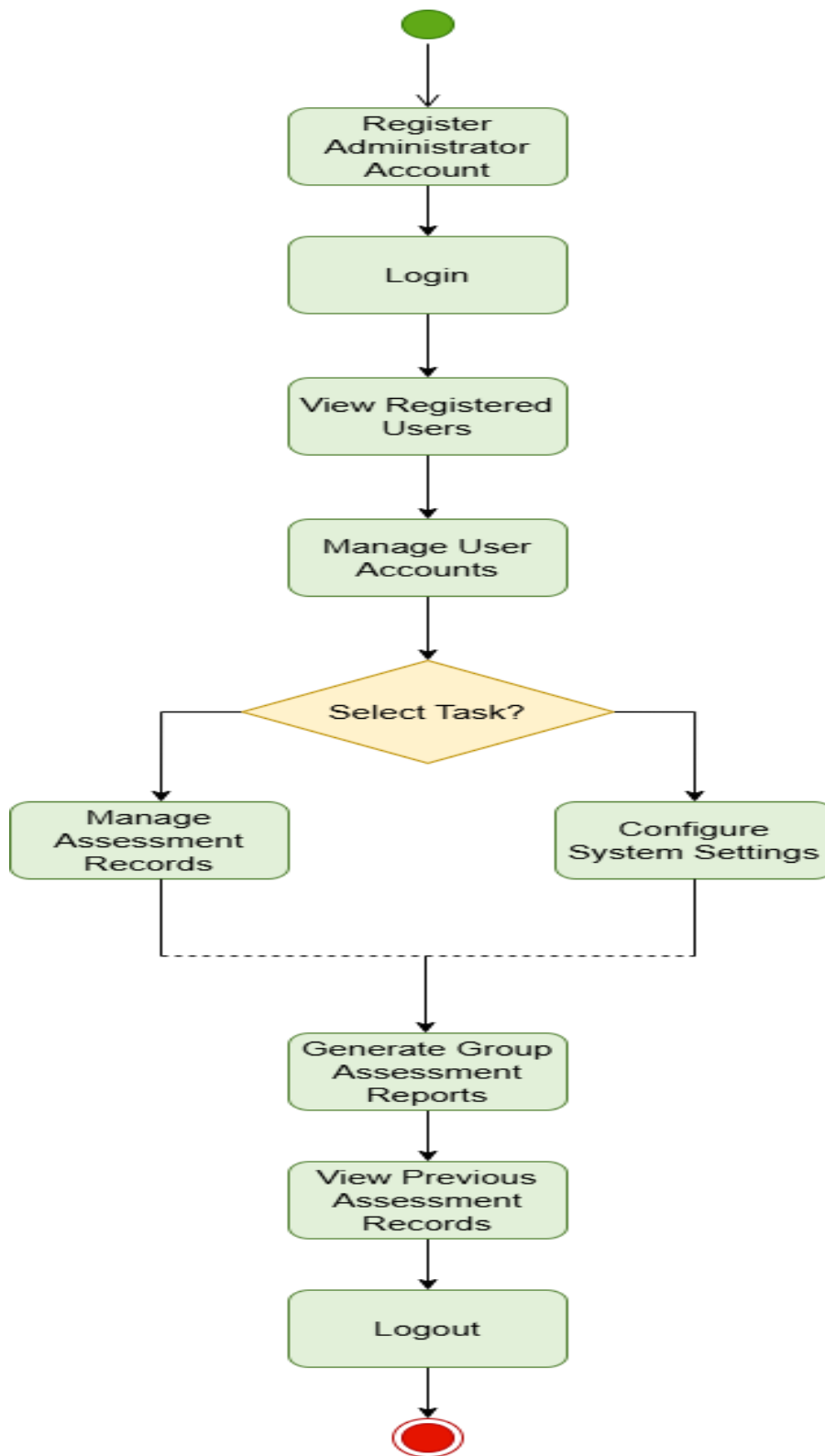
FIG.3 – SYSTEM ADMINISTRATOR ACTIVITY DIAGRAM
